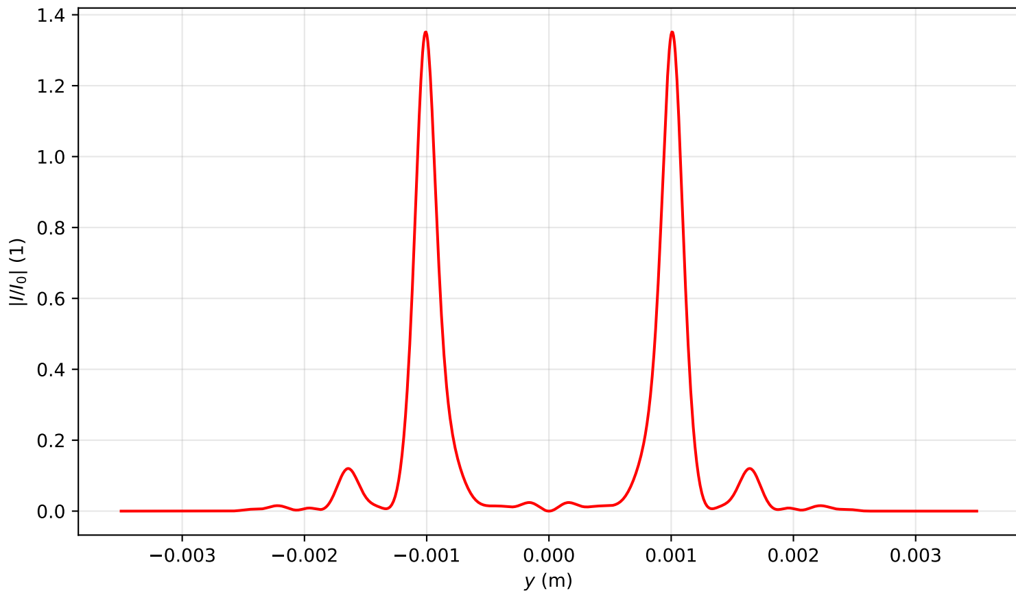
Intensity profile I(x=0, y, z=3.105)/I_0 , P_{in}=17.0\text{Pcr} , artificial time
