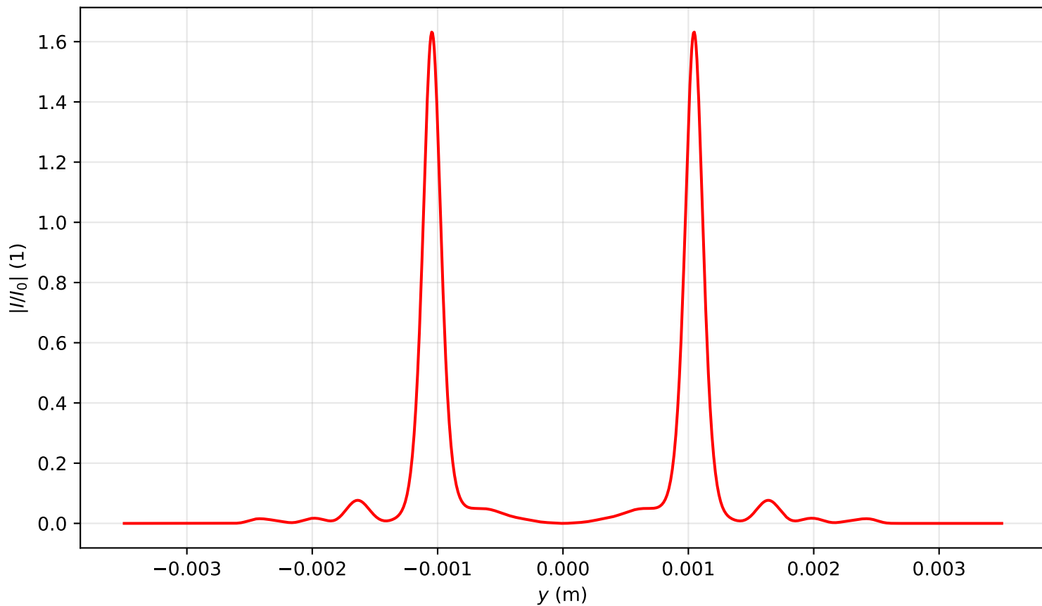
Intensity profile I(x=0, y, z=3.264)/I_0 , P_{in}=17.0\text{Pcr} , artificial time
