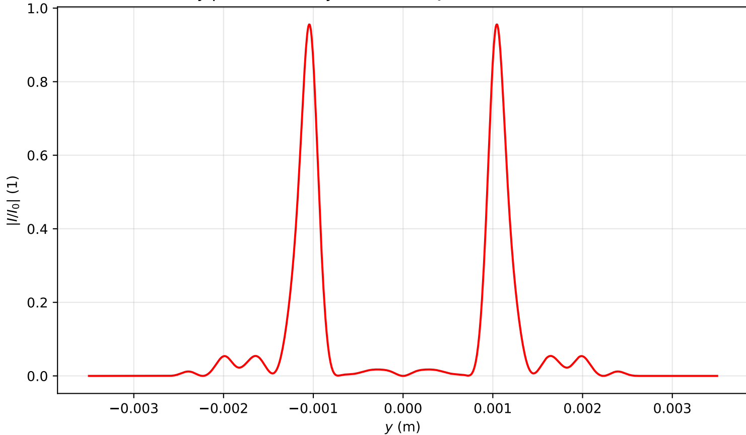
Intensity profile I(x=0, y, z=3.423)/I_0 , P_{in}=17.0P_{cr} , artificial time
