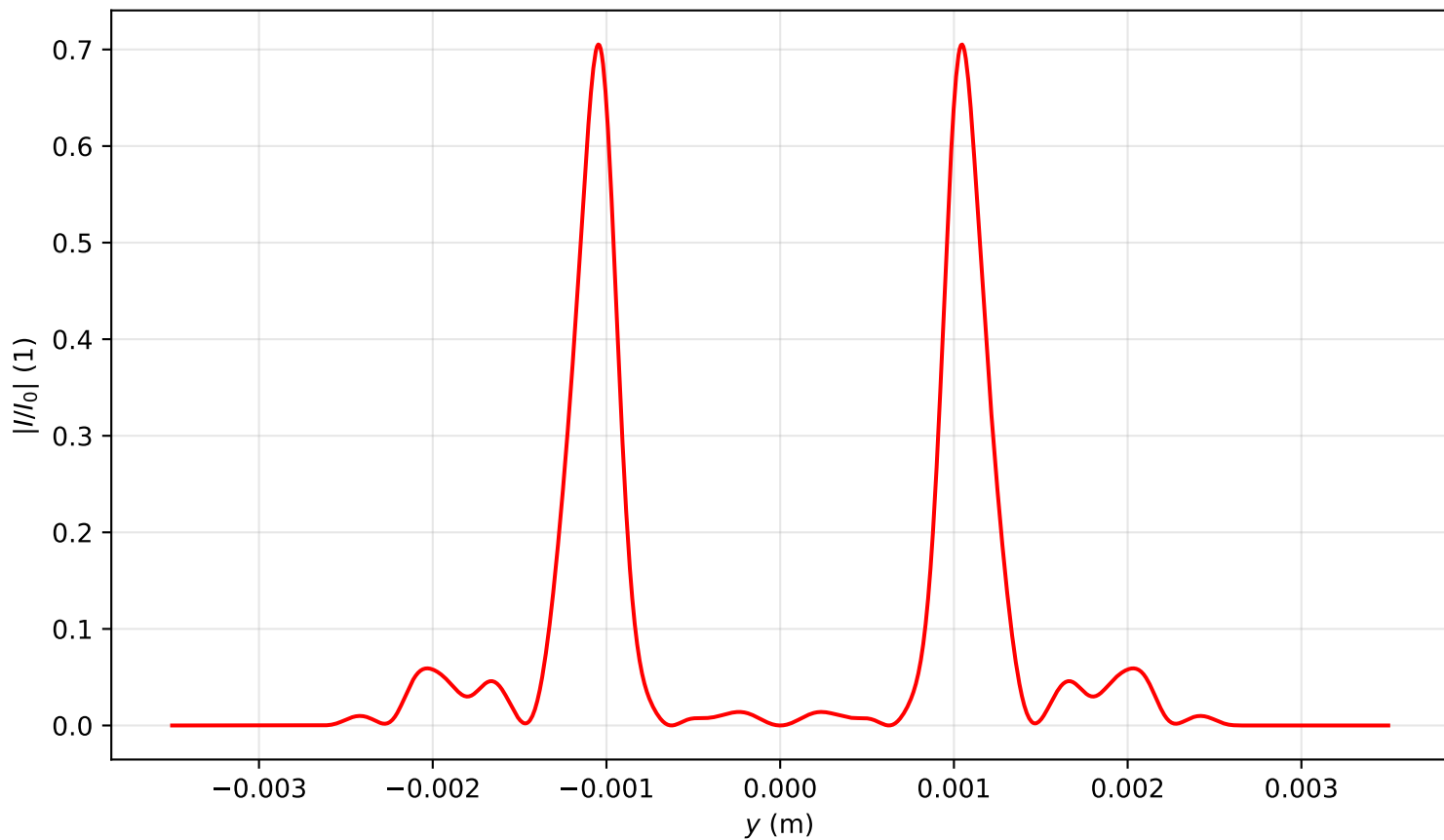
Intensity profile I(x=0, y, z=3.503)/I_0 , P_{in}=17.0P_{cr} , artificial time
