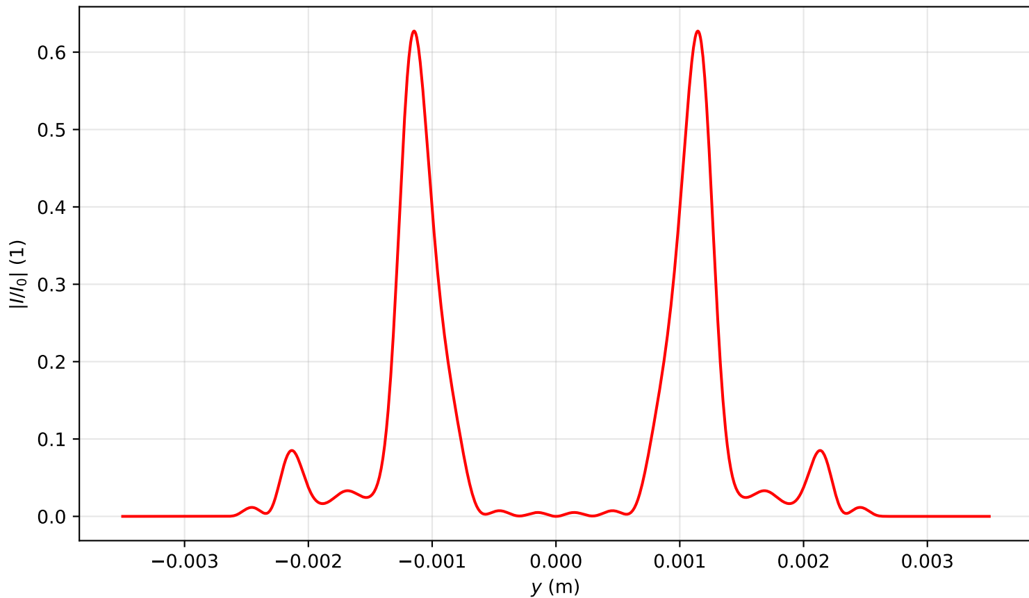
Intensity profile I(x=0, y, z=3.742)/I_0 , P_{in}=17.0\text{Pcr} , artificial time
