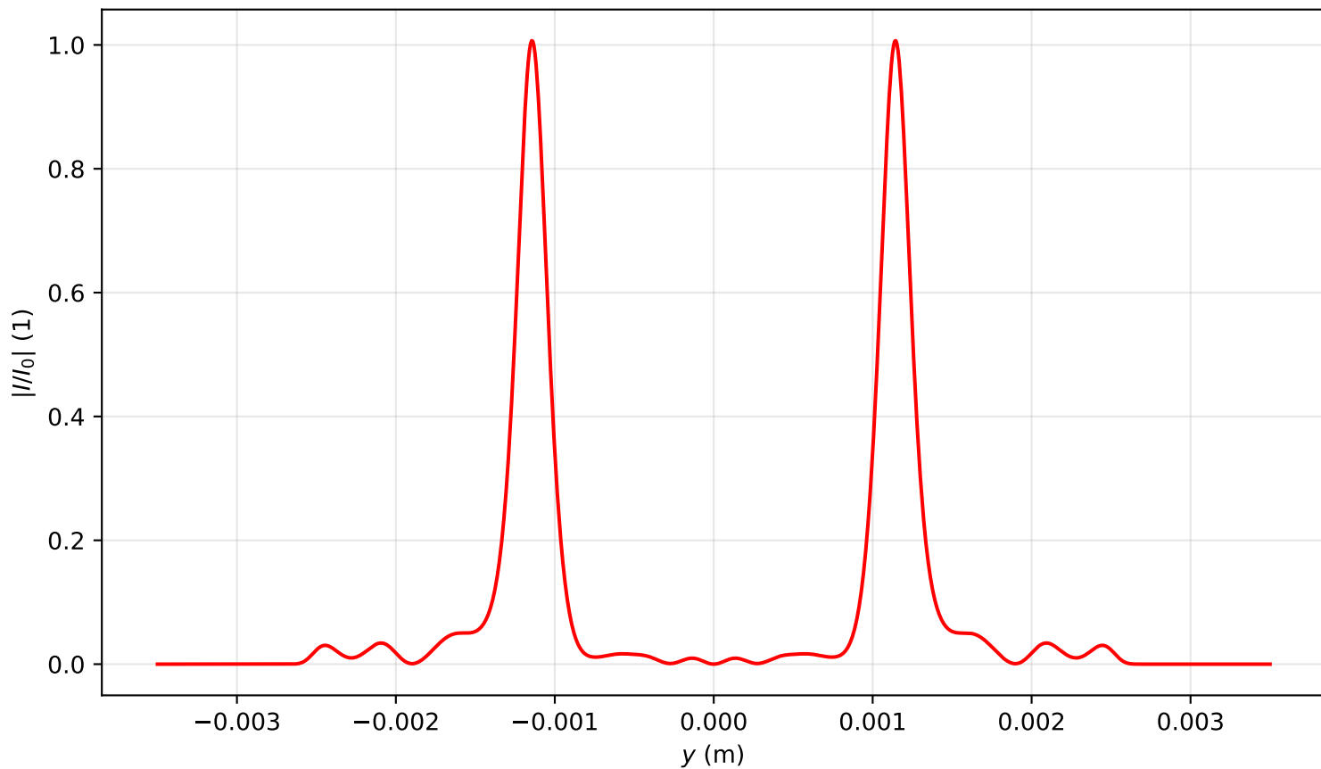
Intensity profile I(x=0, y, z=3.981)/I_0 , P_{in}=17.0P_{cr} , artificial time
