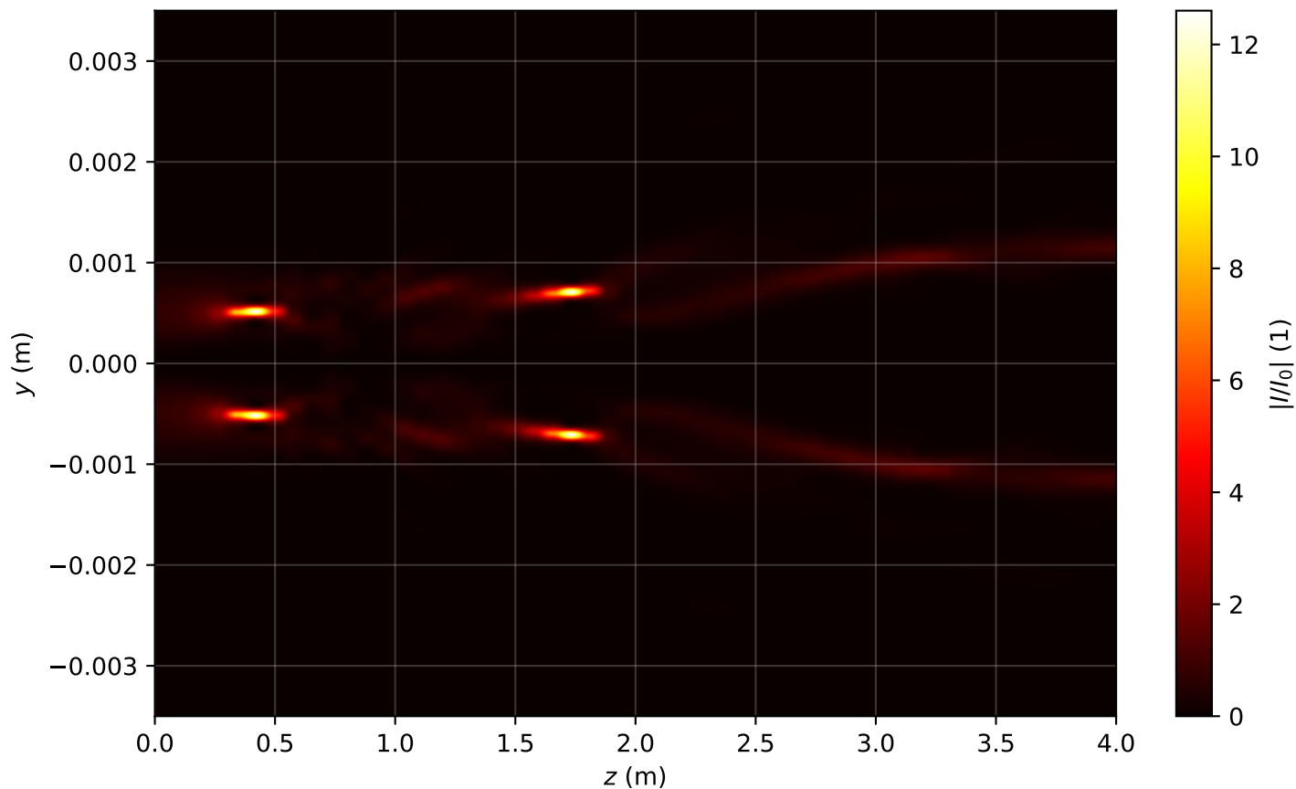
Intensity profile I(x=0, y, z)/I_0 , P_{in}=17.0P_{cr} , artificial time
