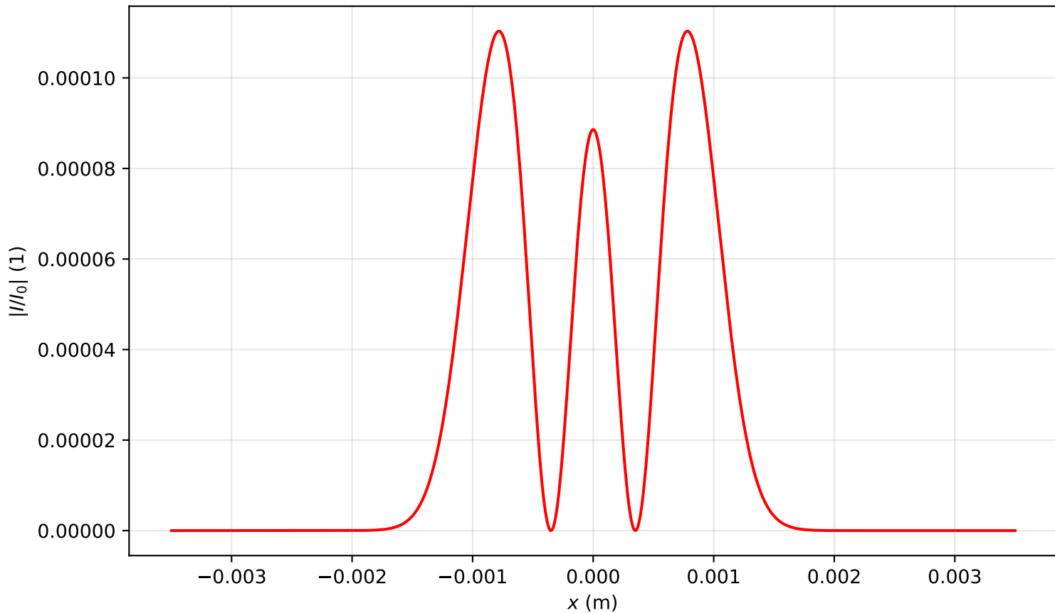
Intensity profile I(x, y = 0, z = 0.080)/I_0 , P_{in}=18.0P_{cr} , artificial time
