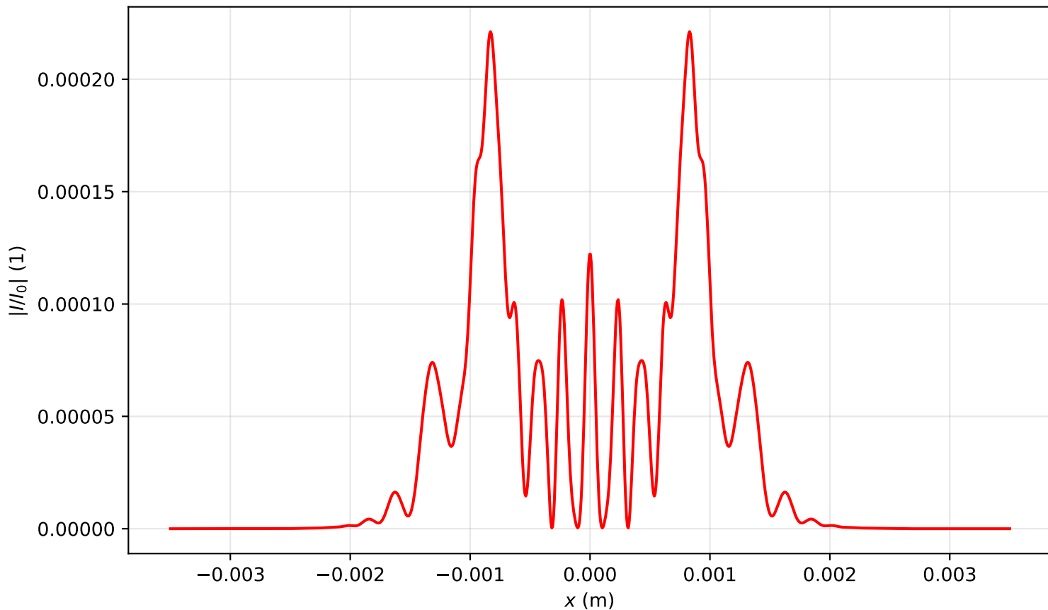
Intensity profile I(x, y = 0, z = 0.478)/I_0 , P_{in}=18.0\text{Pcr} , artificial time
