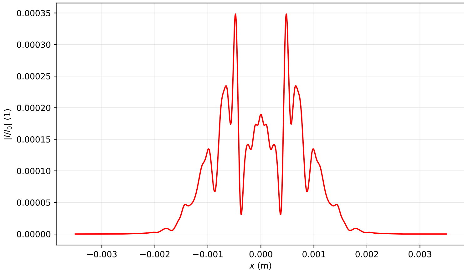
Intensity profile I(x, y = 0, z = 0.557)/I_0 , P_{in}=18.0\text{Pcr} , artificial time
