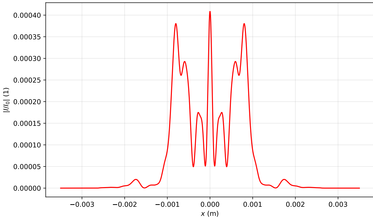
Intensity profile I(x, y = 0, z = 0.716)/I_0 , P_{in}=18.0\text{Pcr} , artificial time
