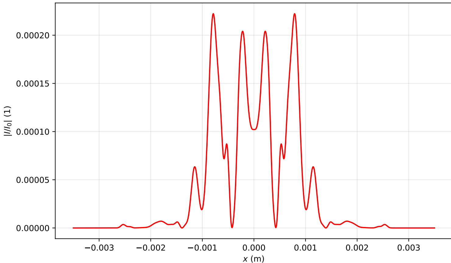
Intensity profile I(x, y = 0, z = 1.035)/I_0 , P_{in}=18.0P_{cr} , artificial time
