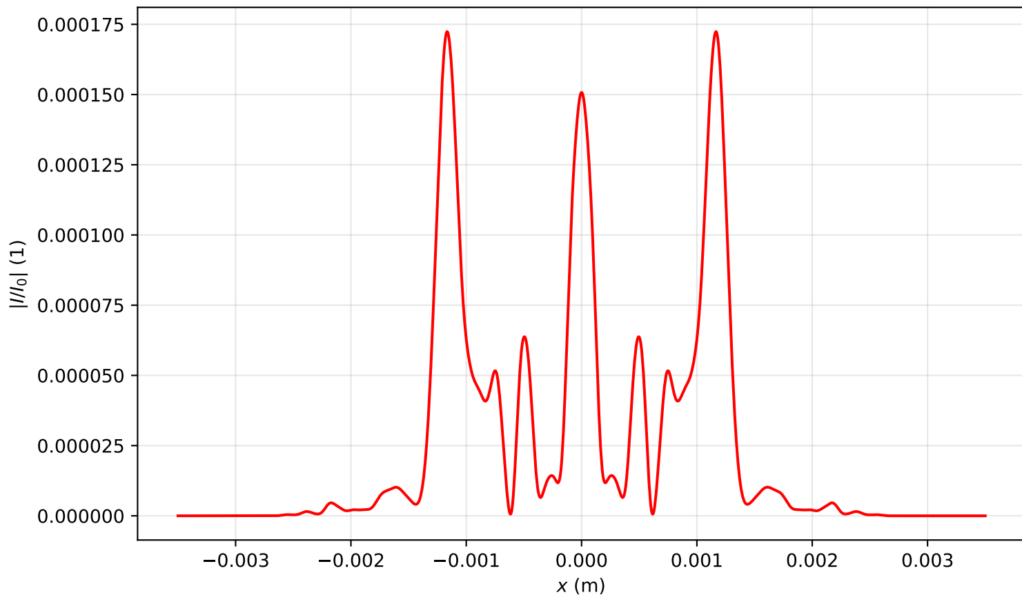
Intensity profile I(x, y = 0, z = 1.194)/I_0 , P_{in}=18.0\text{Pcr} , artificial time
