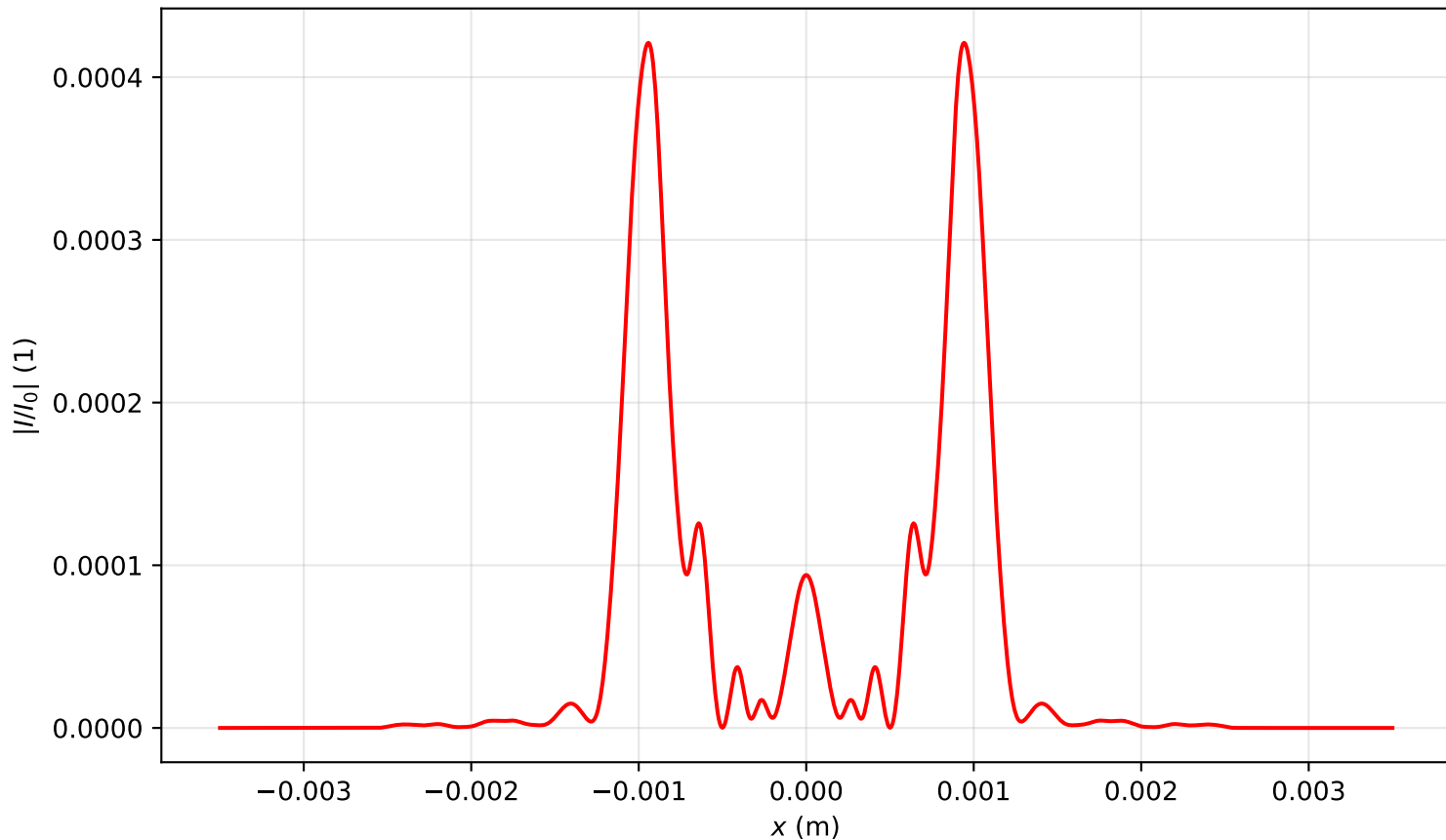
Intensity profile I(x, y = 0, z = 1.274)/I_0 , P_{in}=18.0\text{Pcr} , artificial time
