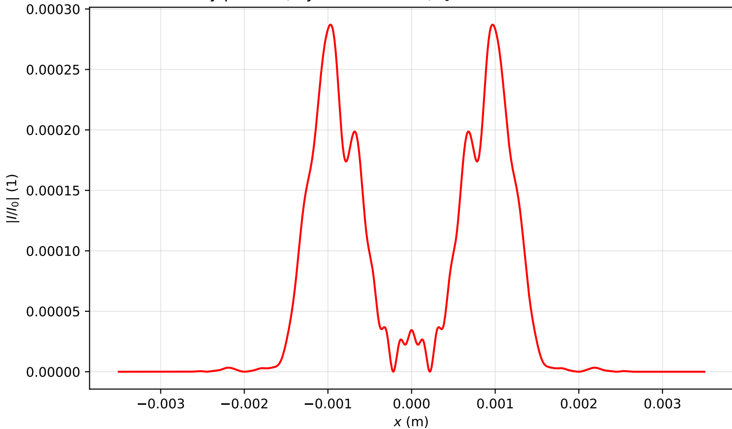
Intensity profile I(x, y = 0, z = 1.433)/I_0 , P_{in}=18.0\text{Pcr} , artificial time
