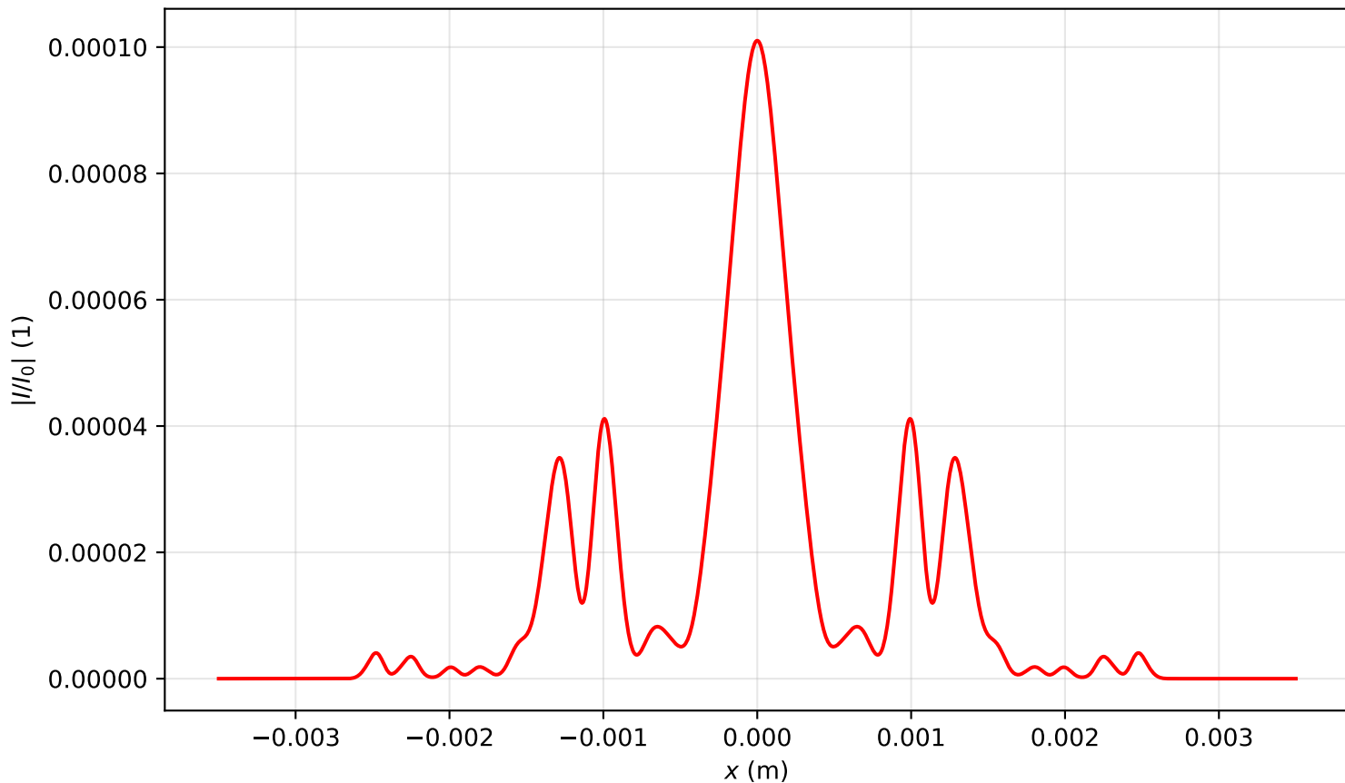
Intensity profile I(x, y = 0, z = 2.070)/I_0 , P_{in}=18.0P_{cr} , artificial time
