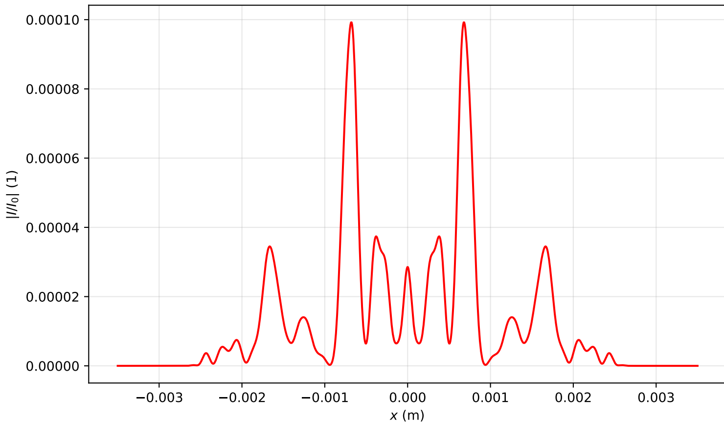
Intensity profile I(x, y = 0, z = 2.468)/I_0 , P_{in}=18.0P_{cr} , artificial time
