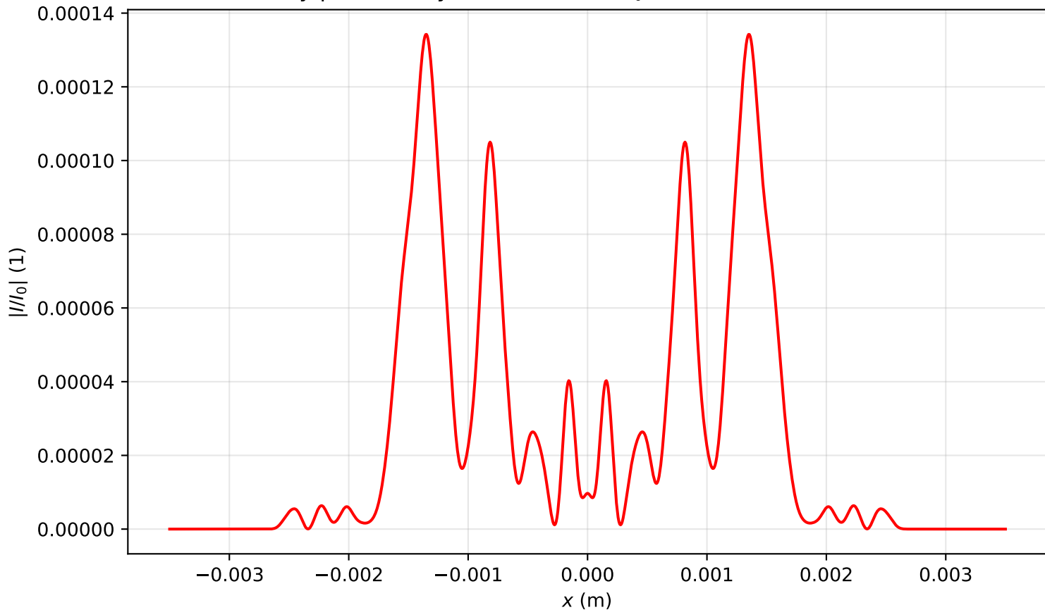
Intensity profile I(x, y = 0, z = 2.627)/I_0 , P_{in}=18.0P_{cr} , artificial time
