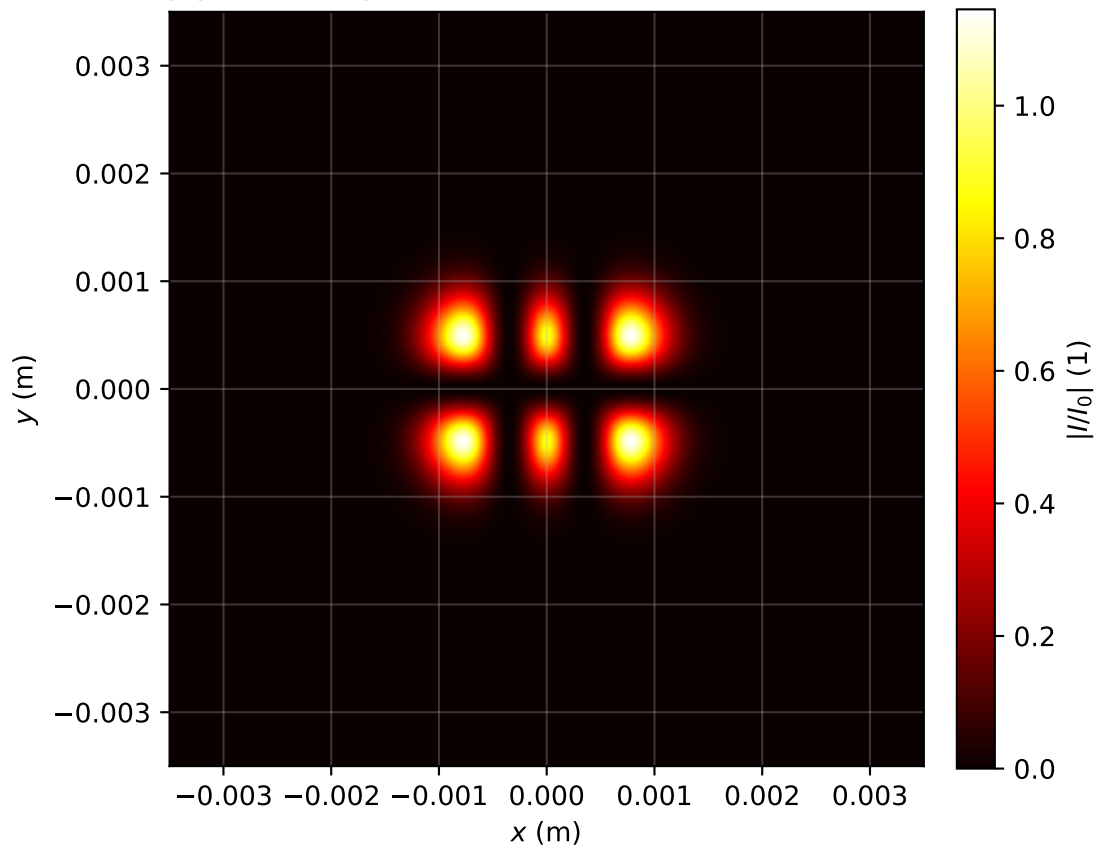
Intensity profile I(x, y, z = 0.080)/I_0 , P_{in}=18.0\text{Pcr} , artificial time
