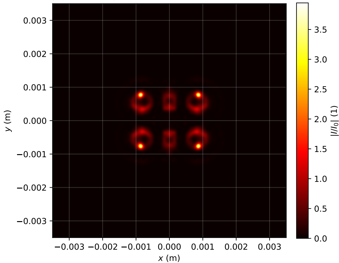
Intensity profile I(x, y, z = 0.557)/I_0 , P_{in}=18.0\text{Pcr} , artificial time
