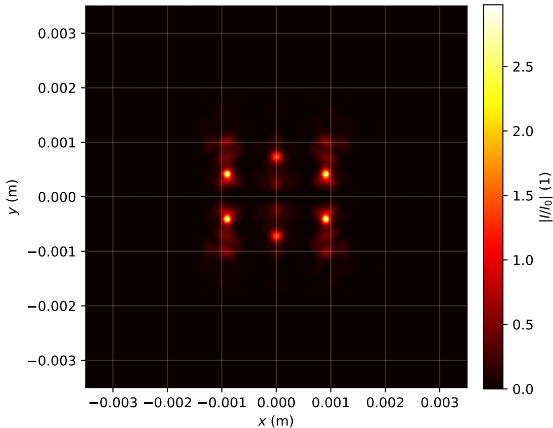
Intensity profile I(x, y, z = 1.115)/I_0 , P_{in}=18.0\text{Pcr} , artificial time
