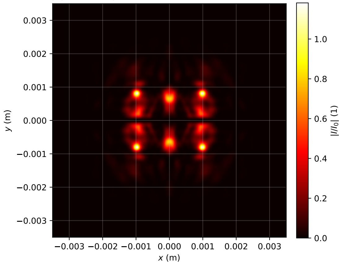
Intensity profile I(x, y, z = 1.353)/I_0 , P_{in}=18.0\text{Pcr} , artificial time
