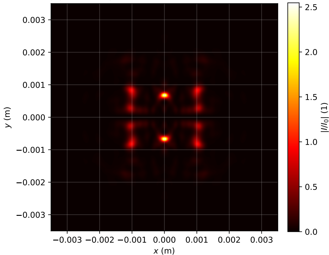
Intensity profile I(x, y, z = 1.513)/I_0 , P_{in}=18.0\text{Pcr} , artificial time
