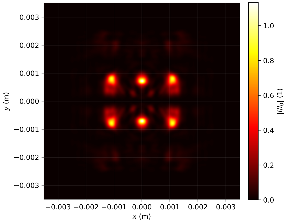
Intensity profile I(x, y, z = 1.831)/I_0 , P_{in}=18.0P_{cr} , artificial time
