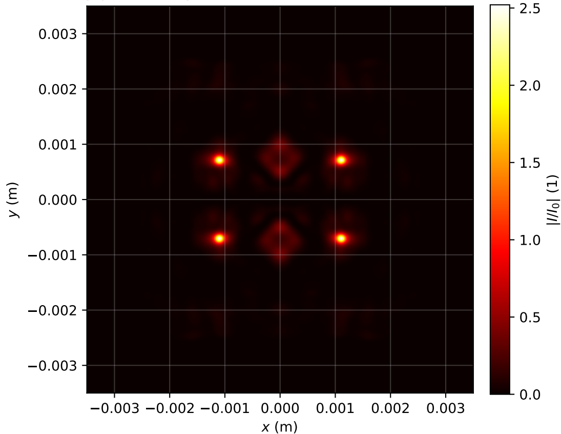
Intensity profile I(x, y, z = 1.990)/I_0 , P_{in}=18.0\text{Pcr} , artificial time
