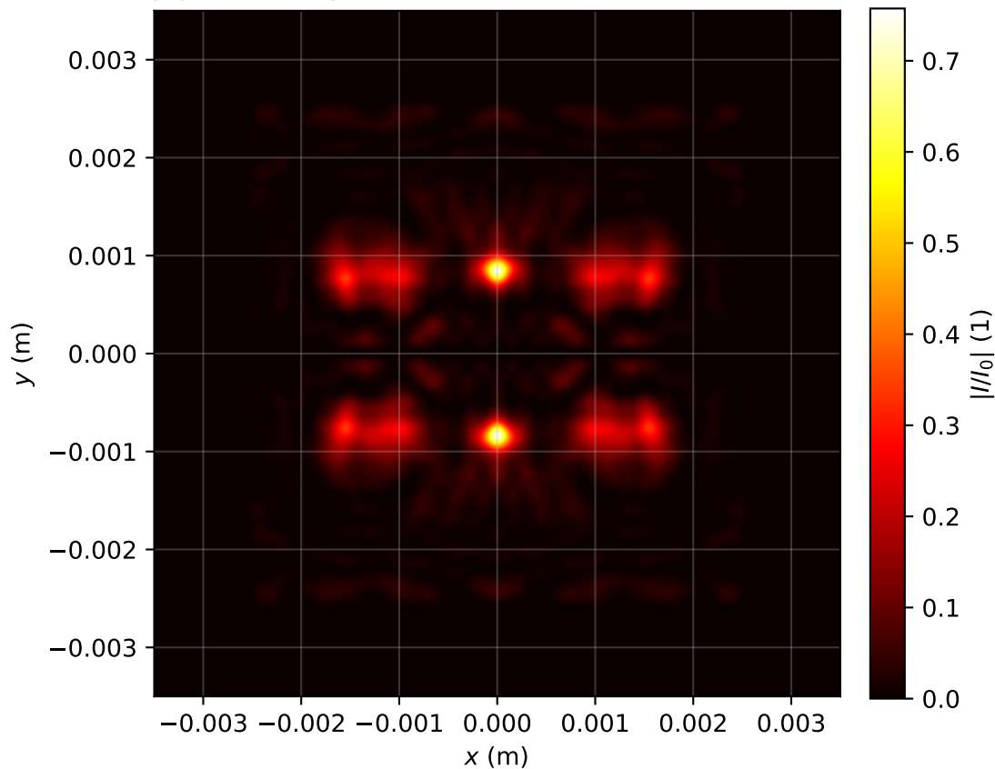
Intensity profile I(x, y, z = 2.627)/I_0 , P_{in}=18.0\text{Pcr} , artificial time
