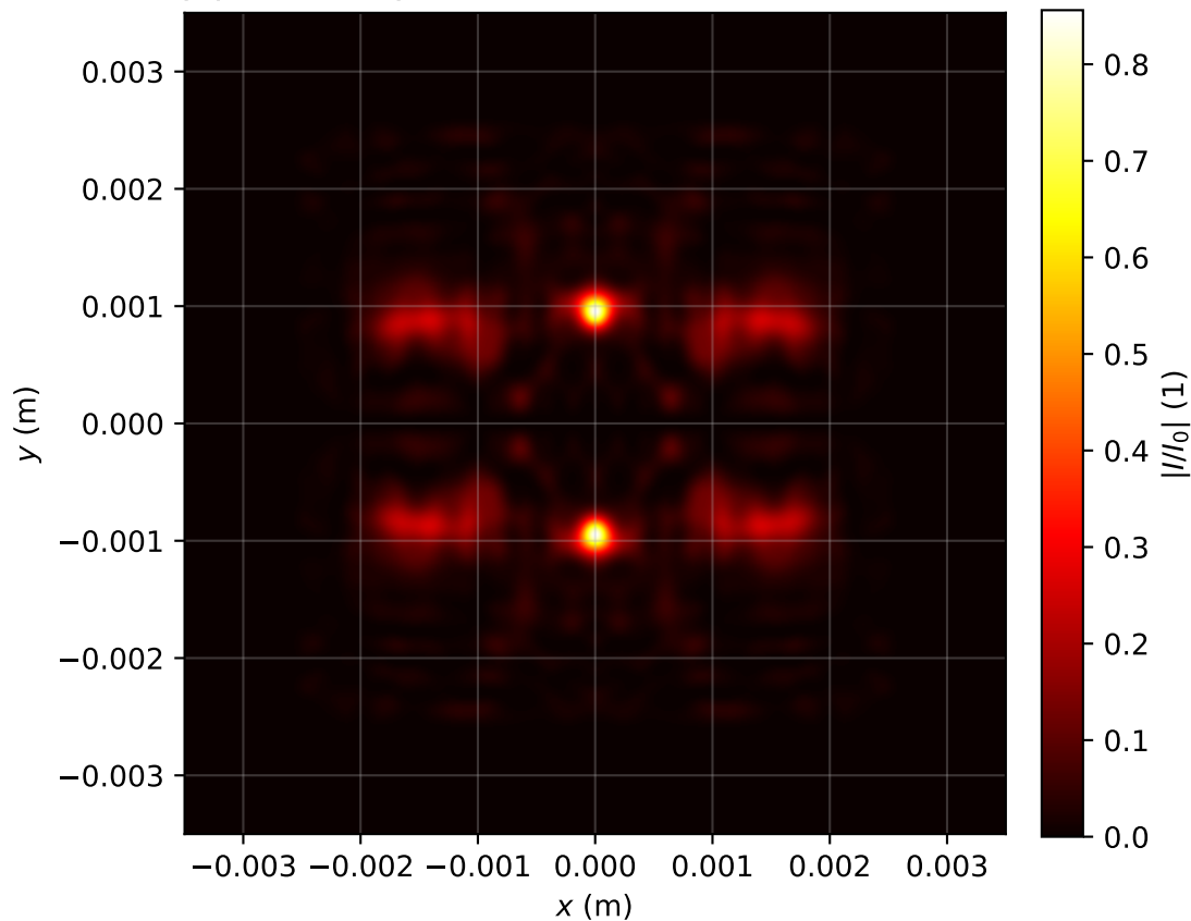
Intensity profile I(x, y, z = 2.866)/I_0 , P_{in}=18.0\text{Pcr} , artificial time
