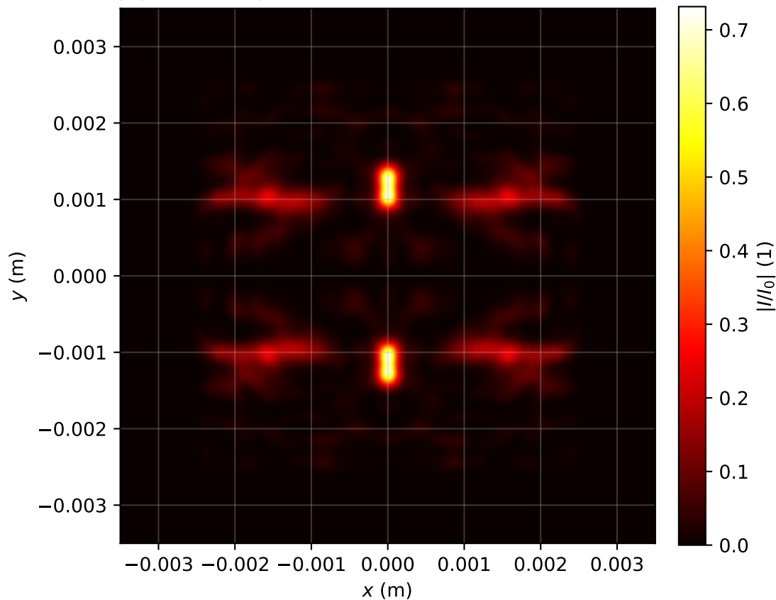
Intensity profile I(x, y, z = 3.423)/I_0 , P_{in}=18.0\text{Pcr} , artificial time
