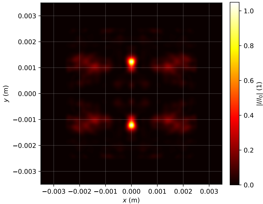
Intensity profile I(x, y, z = 3.582)/I_0 , P_{in}=18.0\text{Pcr} , artificial time
