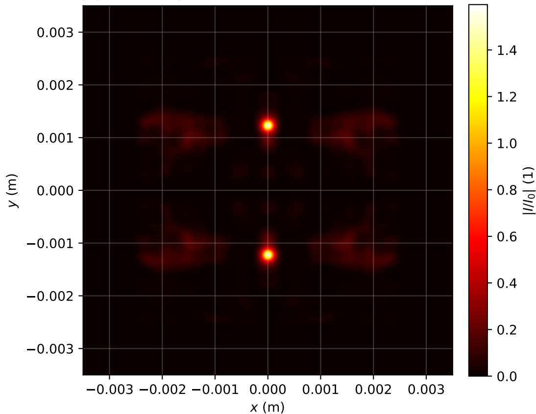
Intensity profile I(x, y, z = 3.662)/I_0 , P_{in}=18.0\text{Pcr} , artificial time
