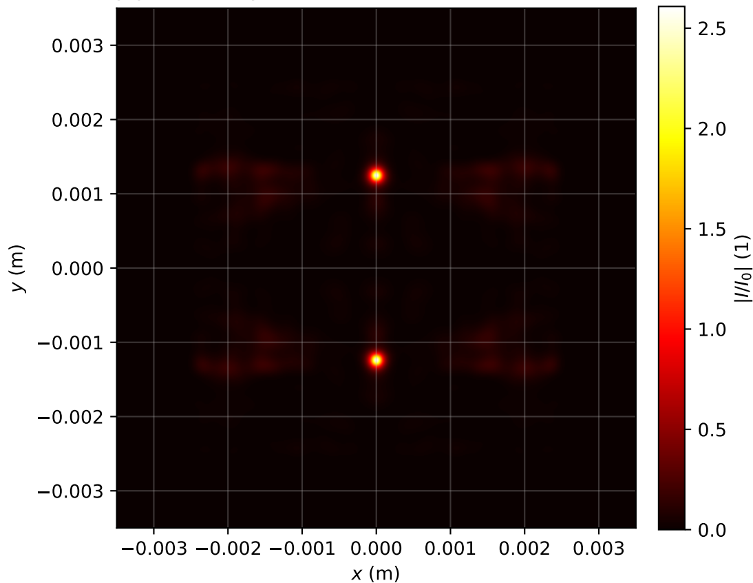
Intensity profile I(x, y, z = 3.742)/I_0 , P_{in}=18.0\text{Pcr} , artificial time
