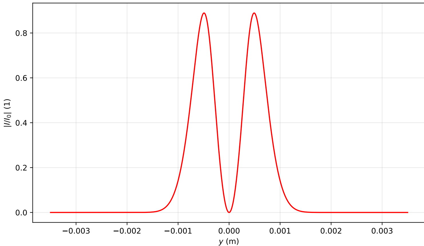
Intensity profile I(x=0, y, z=0.080)/I_0 , P_{in}=18.0P_{cr} , artificial time
