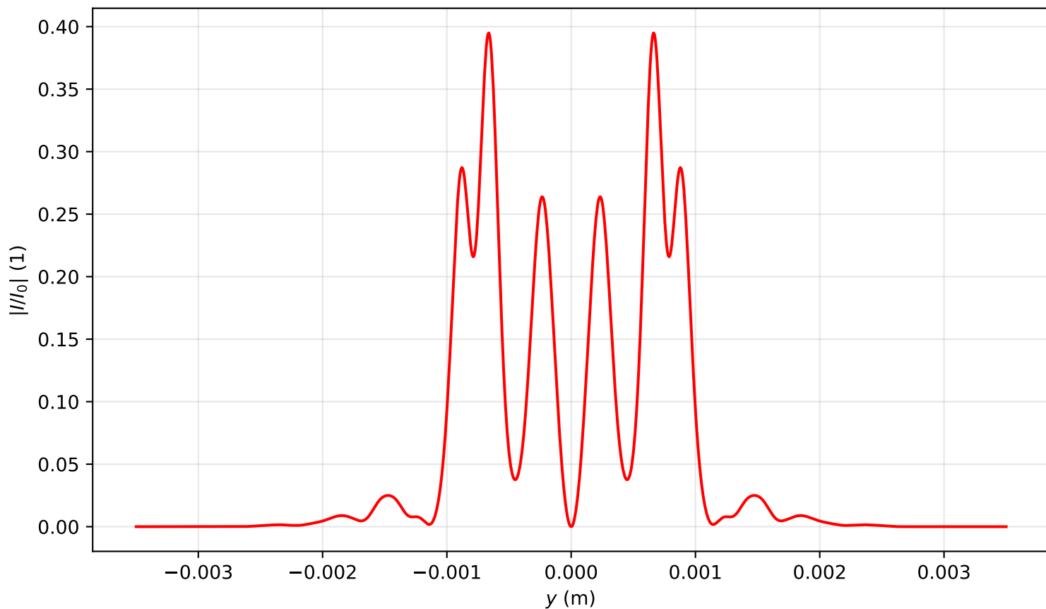
Intensity profile I(x = 0, y, z = 0.796)/I_0 , P_{in}=18.0P_{cr} , artificial time
