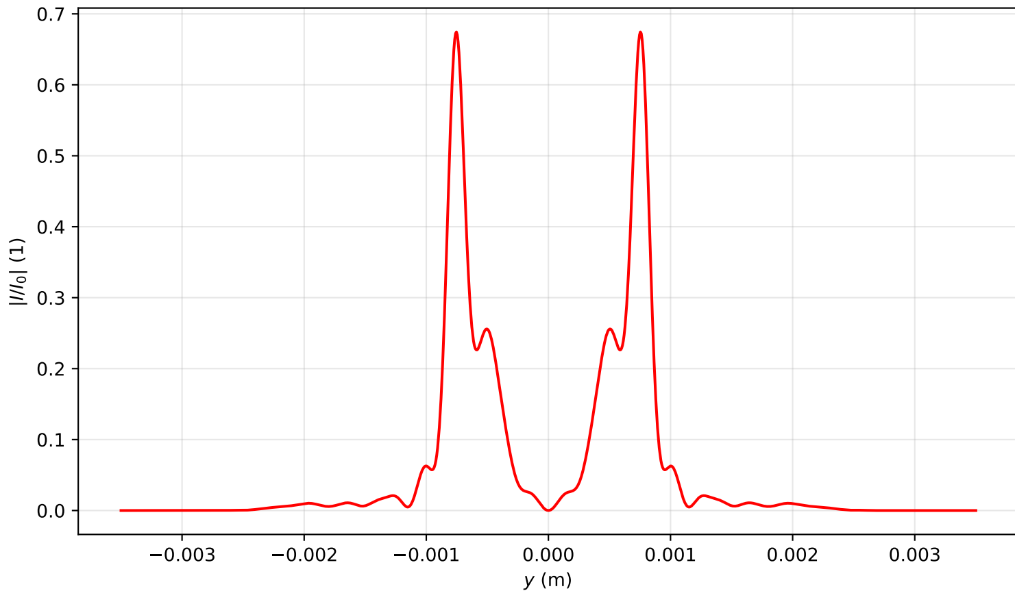
Intensity profile I(x=0, y, z=0.876)/I_0 , P_{in}=18.0\text{Pcr} , artificial time
