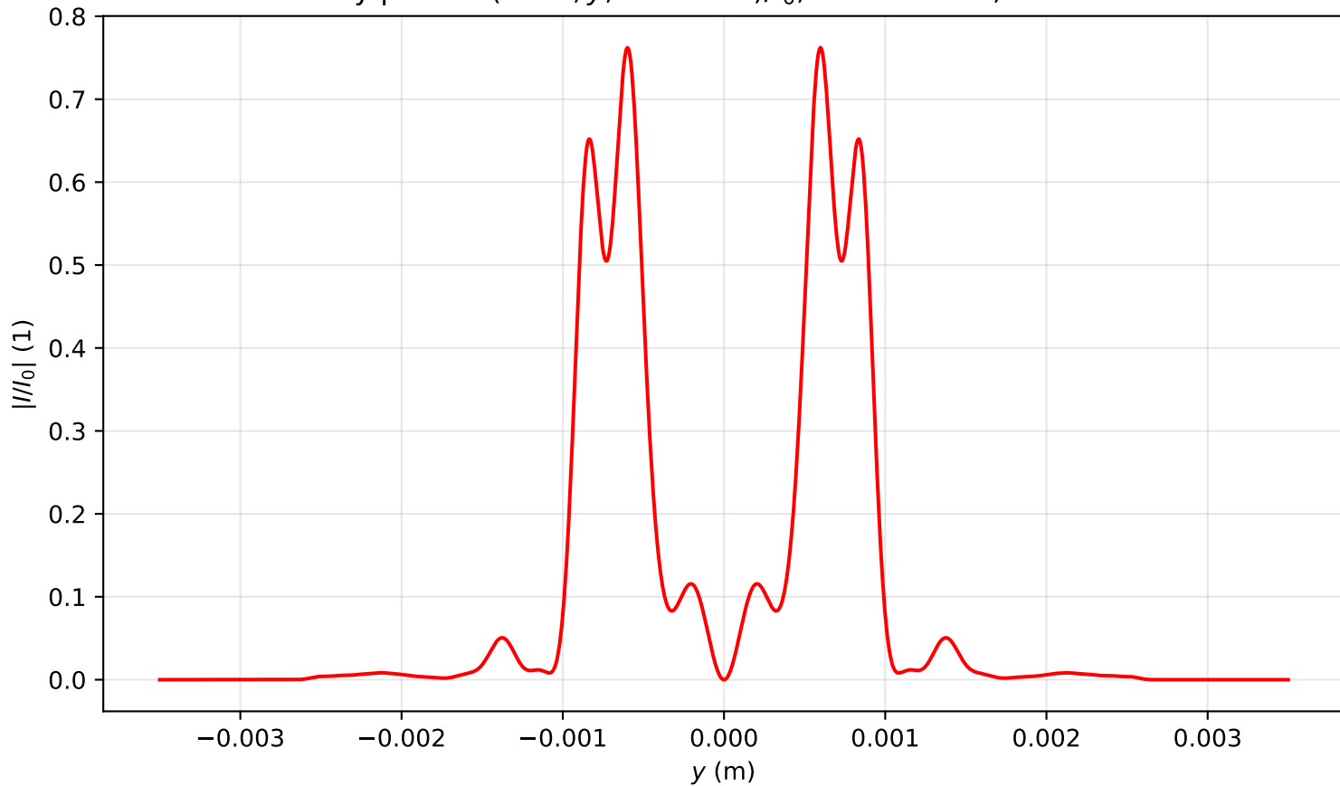
Intensity profile I(x=0, y, z=0.955)/I_0 , P_{in}=18.0\text{Pcr} , artificial time
