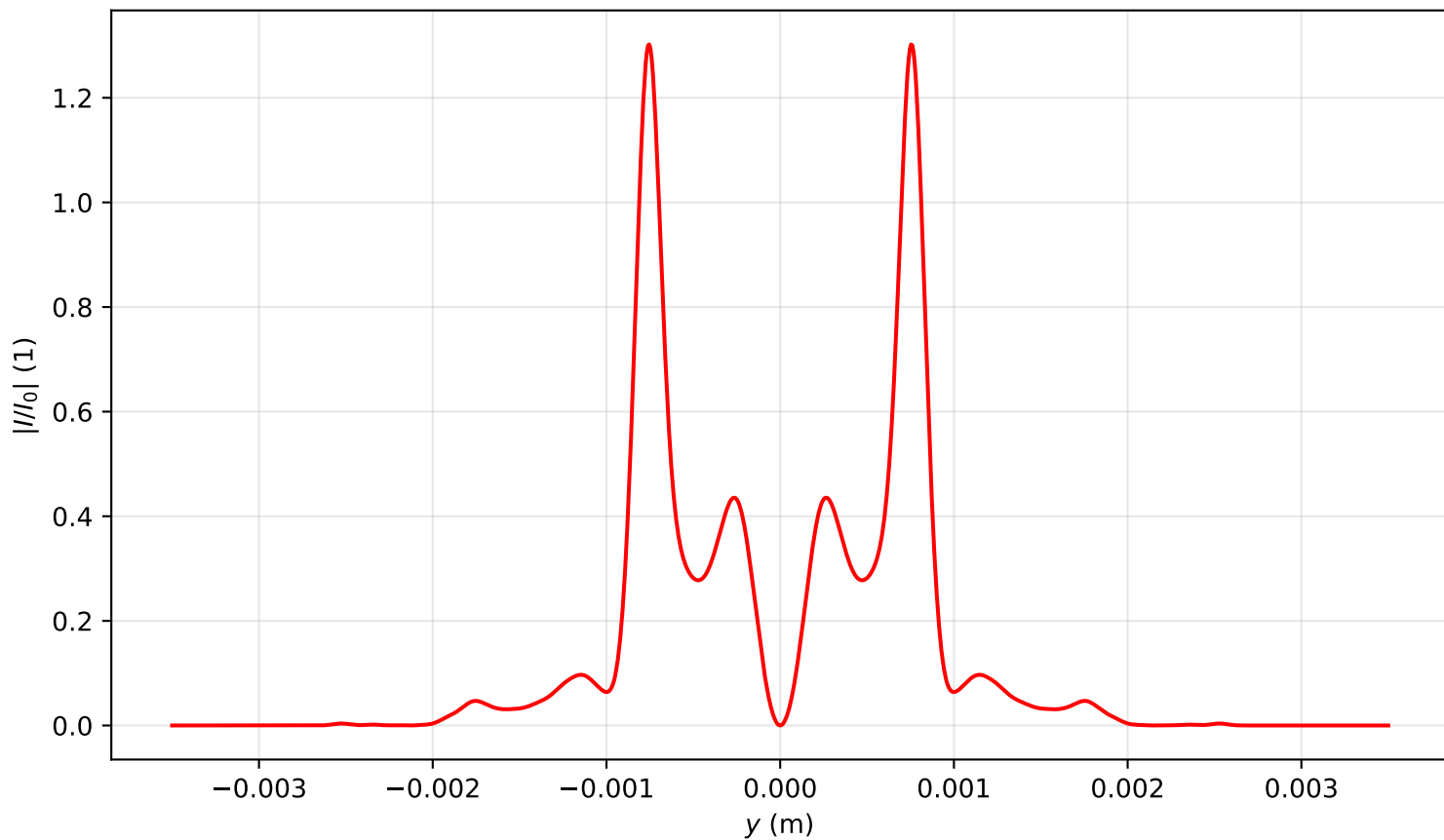
Intensity profile I(x=0, y, z=1.194)/I_0 , P_{in}=18.0\text{Pcr} , artificial time
