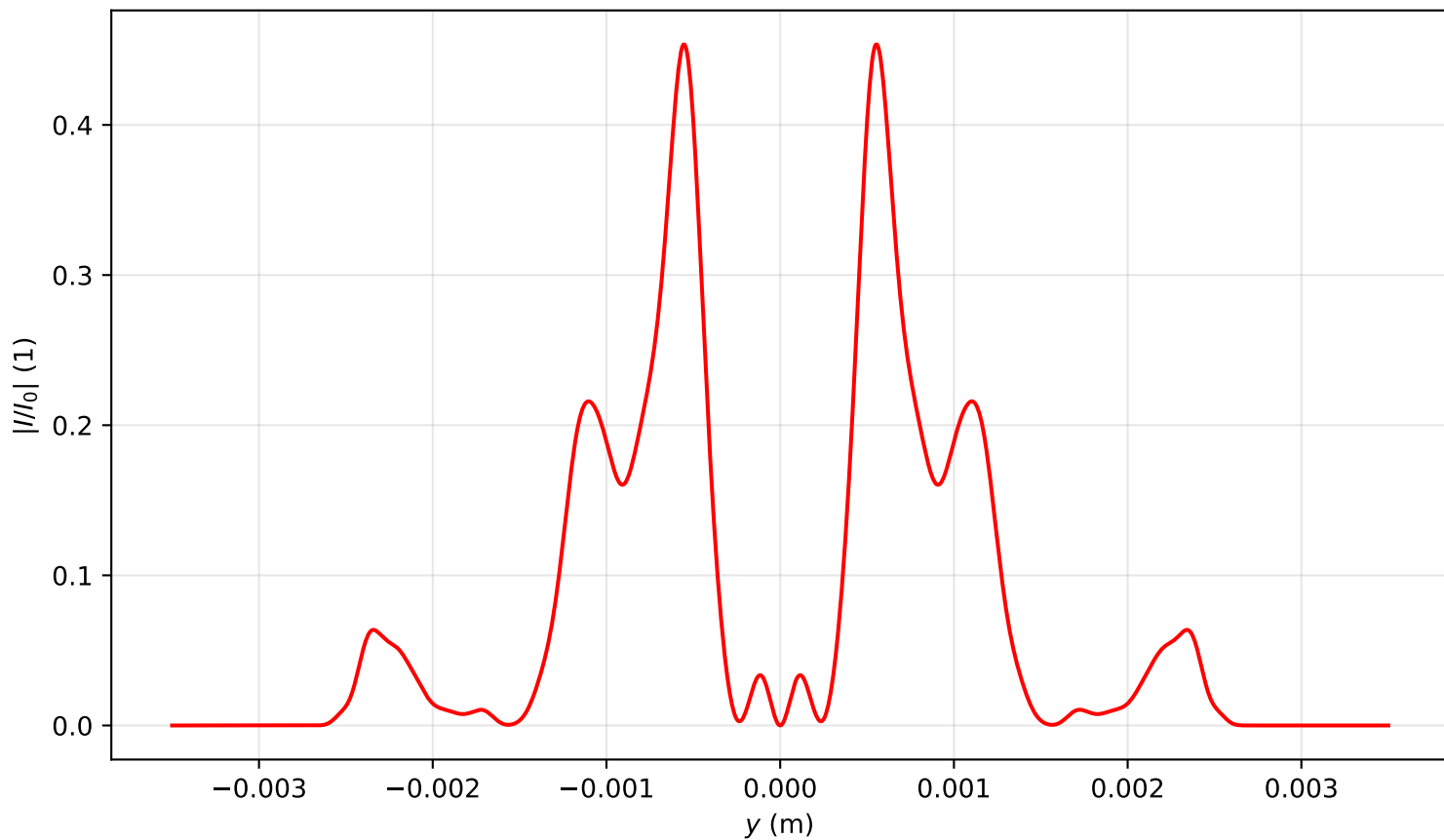
Intensity profile I(x=0, y, z=2.149)/I_0 , P_{in}=18.0P_{cr} , artificial time
