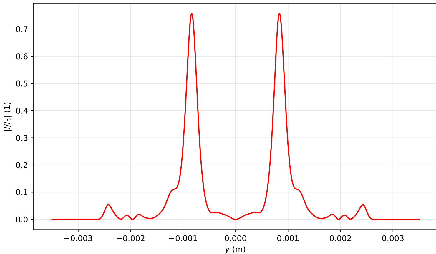
Intensity profile I(x=0, y, z=2.627)/I_0 , P_{in}=18.0\text{Pcr} , artificial time
