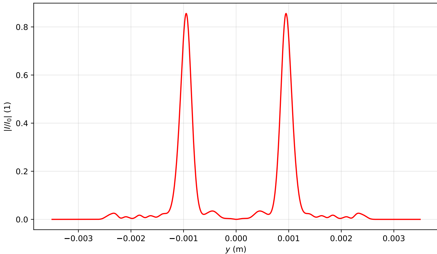
Intensity profile I(x=0, y, z=2.866)/I_0 , P_{in}=18.0\text{Pcr} , artificial time
