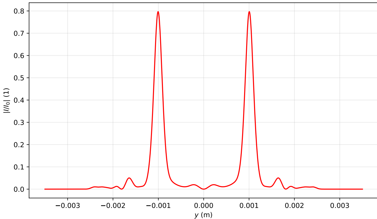
Intensity profile I(x=0, y, z=2.946)/I_0 , P_{in}=18.0\text{Pcr} , artificial time
