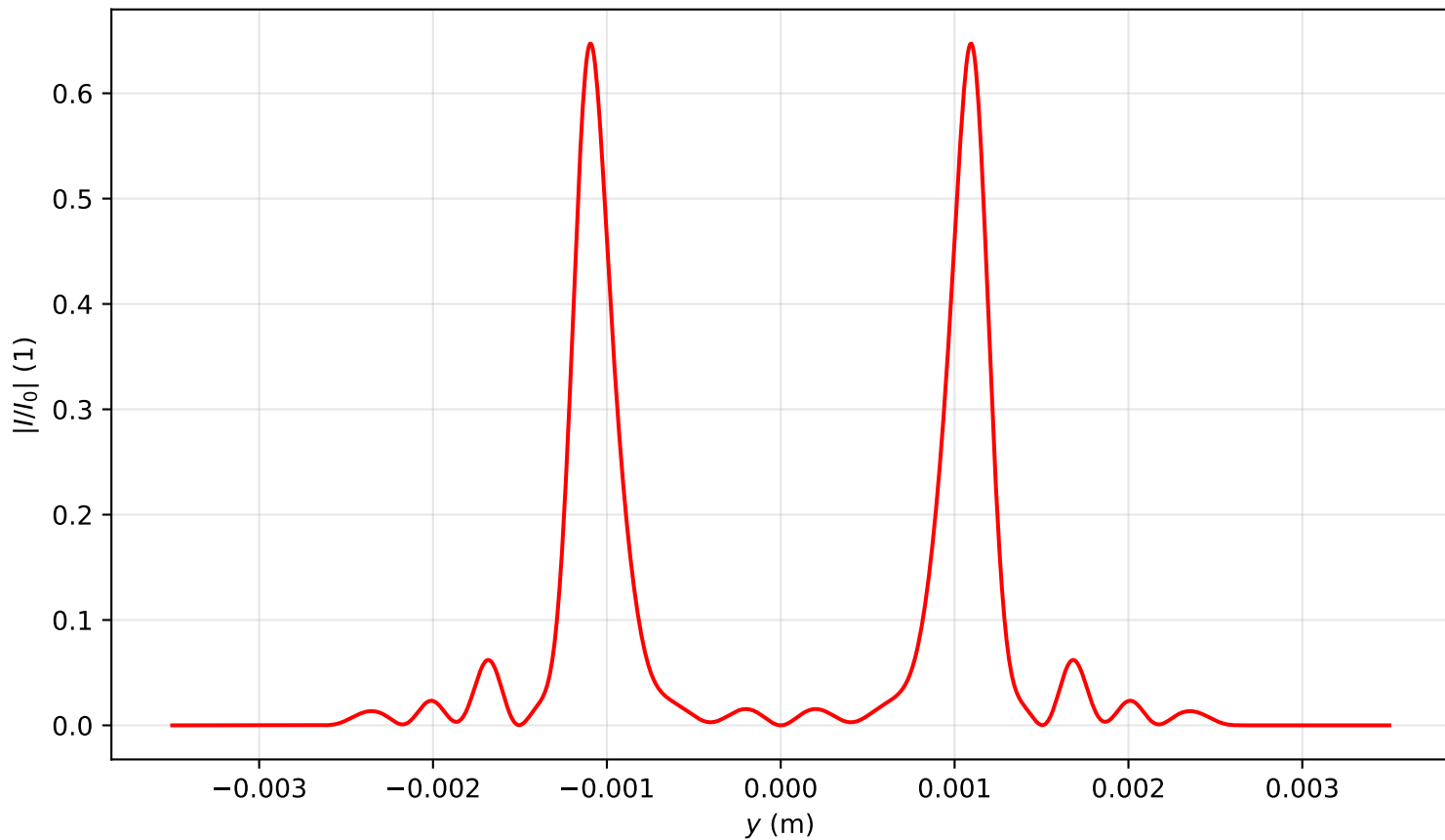
Intensity profile I(x=0, y, z=3.105)/I_0 , P_{in}=18.0\text{Pcr} , artificial time
