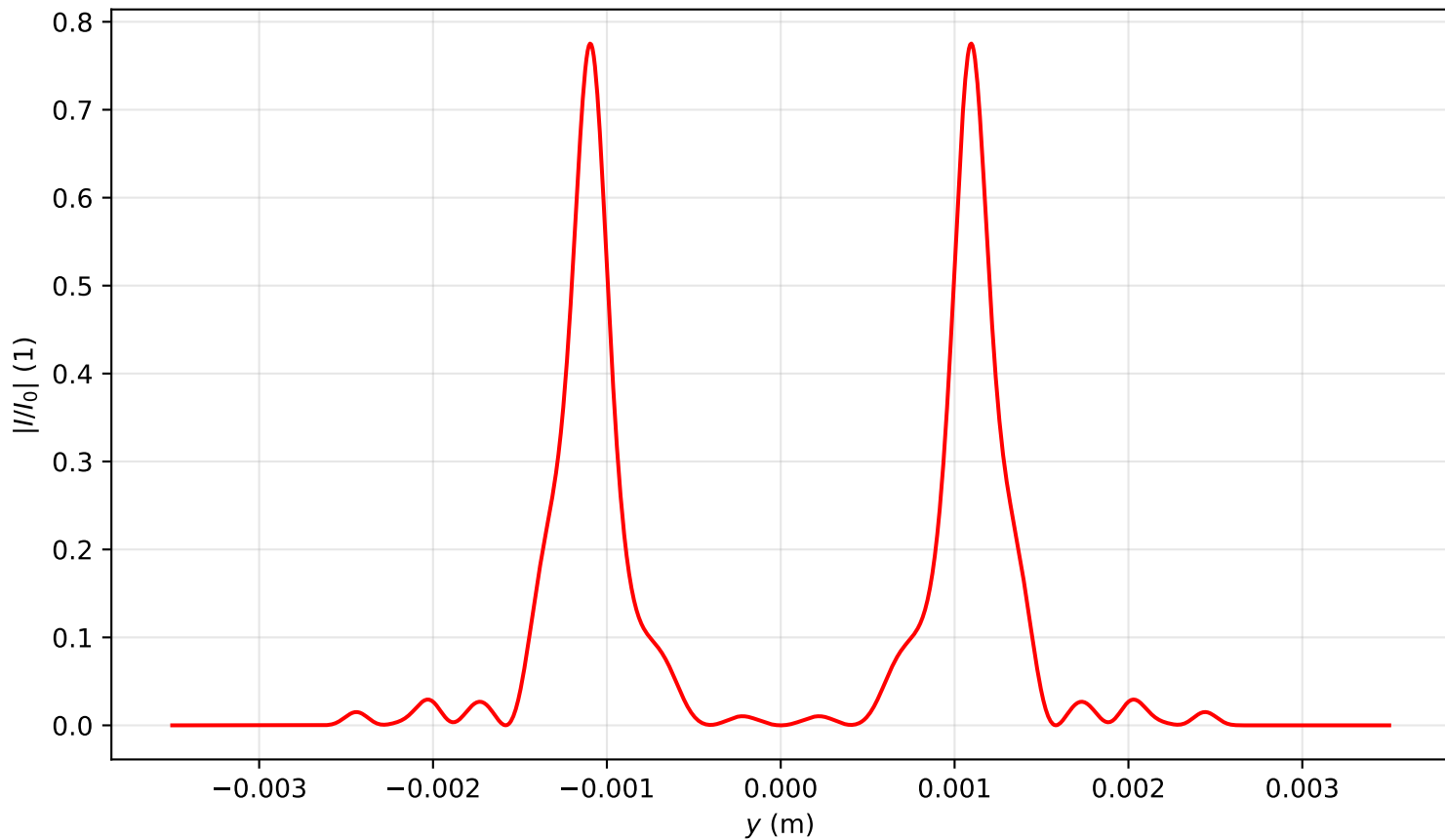
Intensity profile I(x=0, y, z=3.264)/I_0 , P_{in}=18.0\text{Pcr} , artificial time
