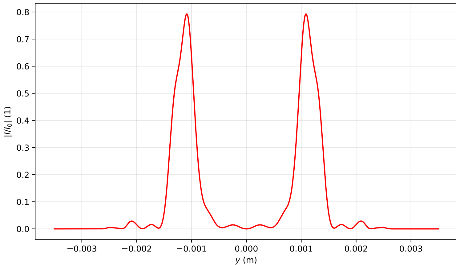
Intensity profile I(x=0, y, z=3.344)/I_0 , P_{in}=18.0P_{cr} , artificial time
