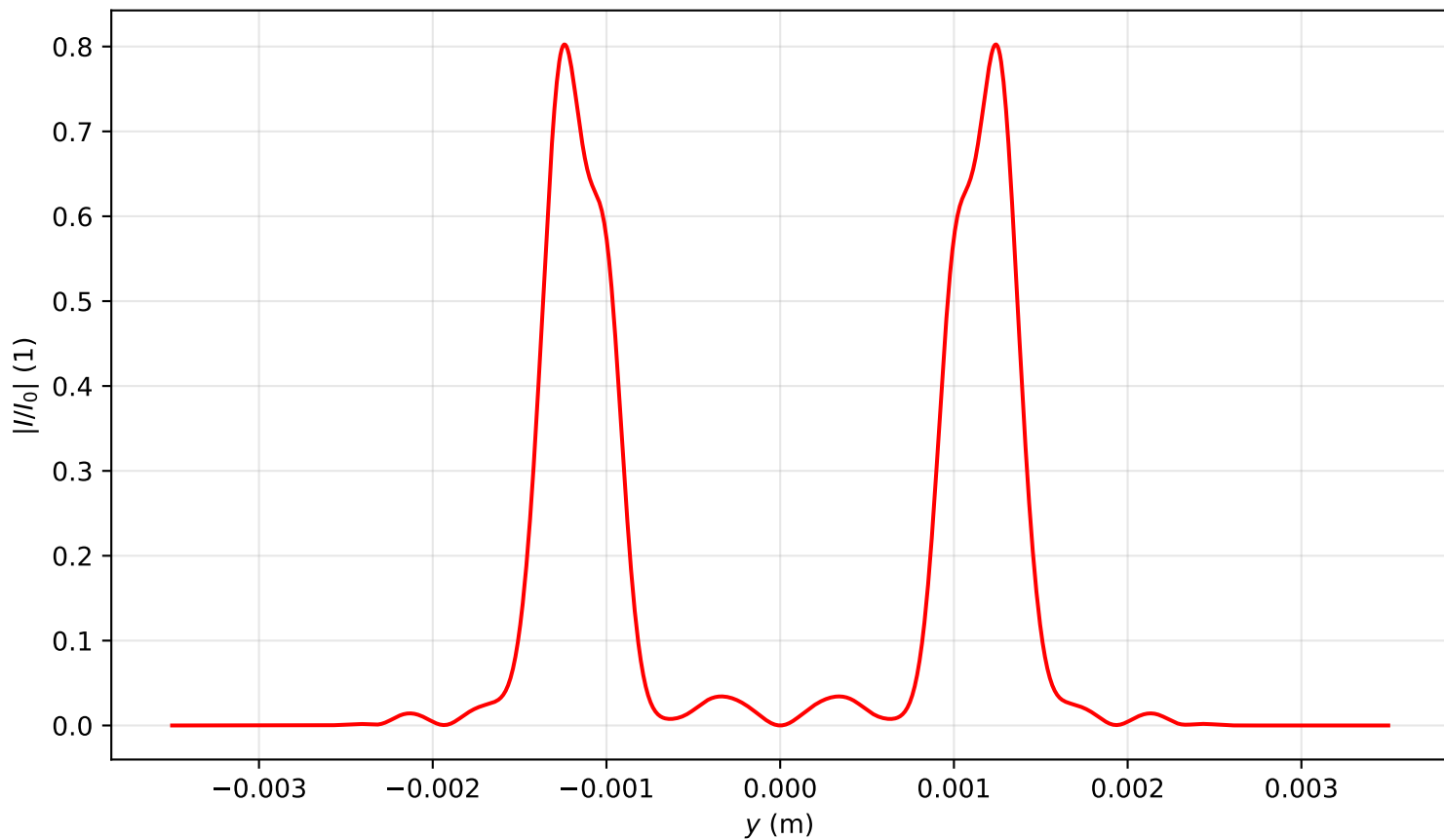
Intensity profile I(x=0, y, z=3.503)/I_0 , P_{in}=18.0\text{Pcr} , artificial time
