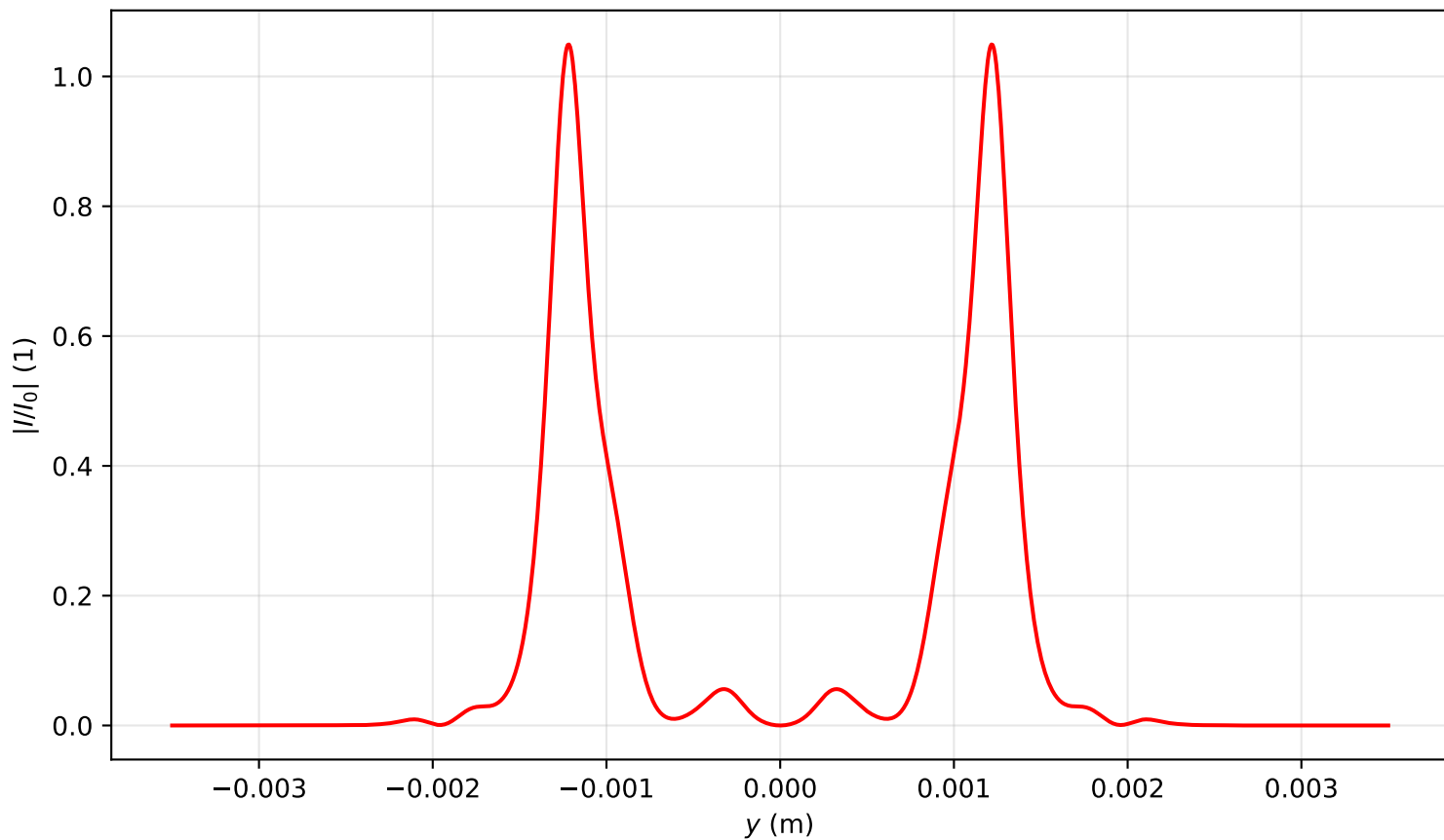
Intensity profile I(x=0, y, z=3.582)/I_0 , P_{in}=18.0\text{Pcr} , artificial time
