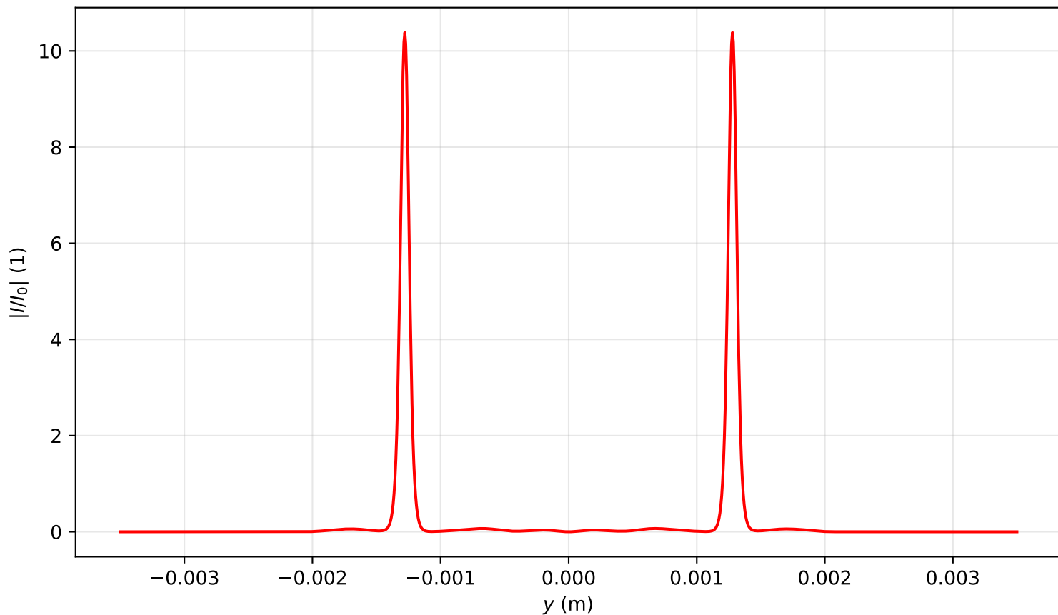
Intensity profile I(x=0, y, z=3.901)/I_0 , P_{in}=18.0\text{Pcr} , artificial time
