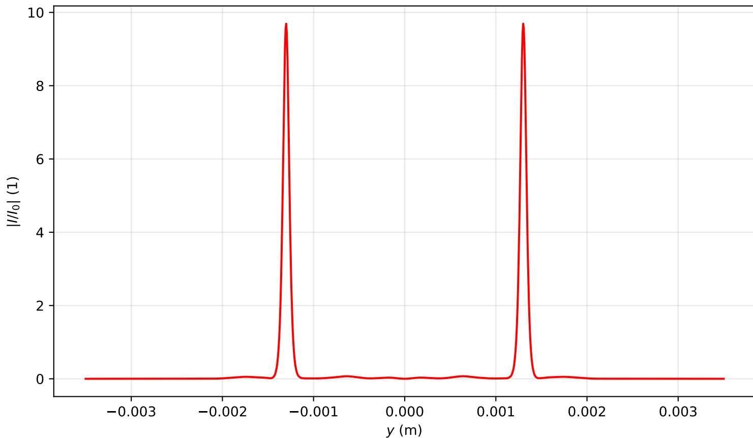
Intensity profile I(x=0, y, z=3.981)/I_0 , P_{in}=18.0\text{Pcr} , artificial time
