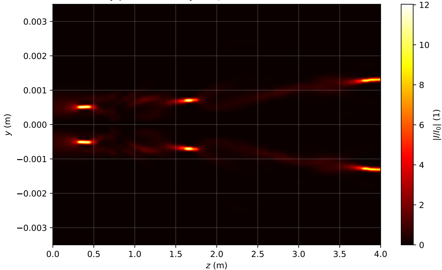
Intensity profile I(x = 0, y, z)/I_0 , P_{in}=18.0P_{cr} , artificial time
