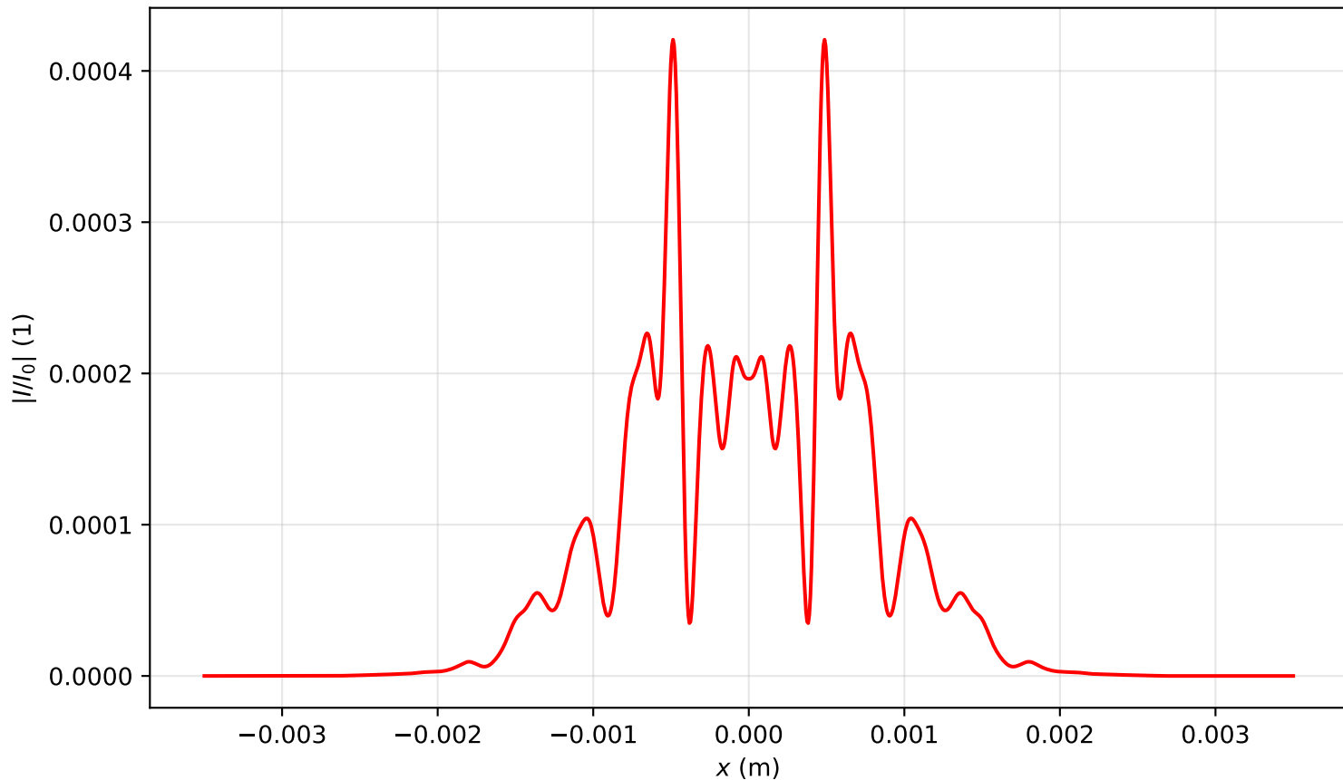
Intensity profile I(x, y = 0, z = 0.557)/I_0 , \text{Pin}=19.0\text{Pcr} , artificial time
