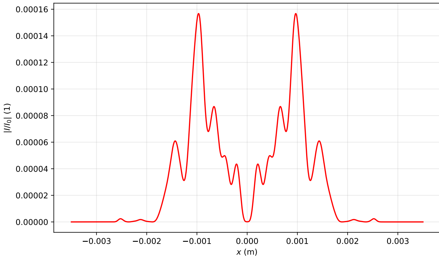
Intensity profile I(x, y = 0, z = 1.513)/I_0 , P_{in}=19.0P_{cr} , artificial time
